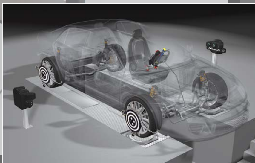
Floor installation
